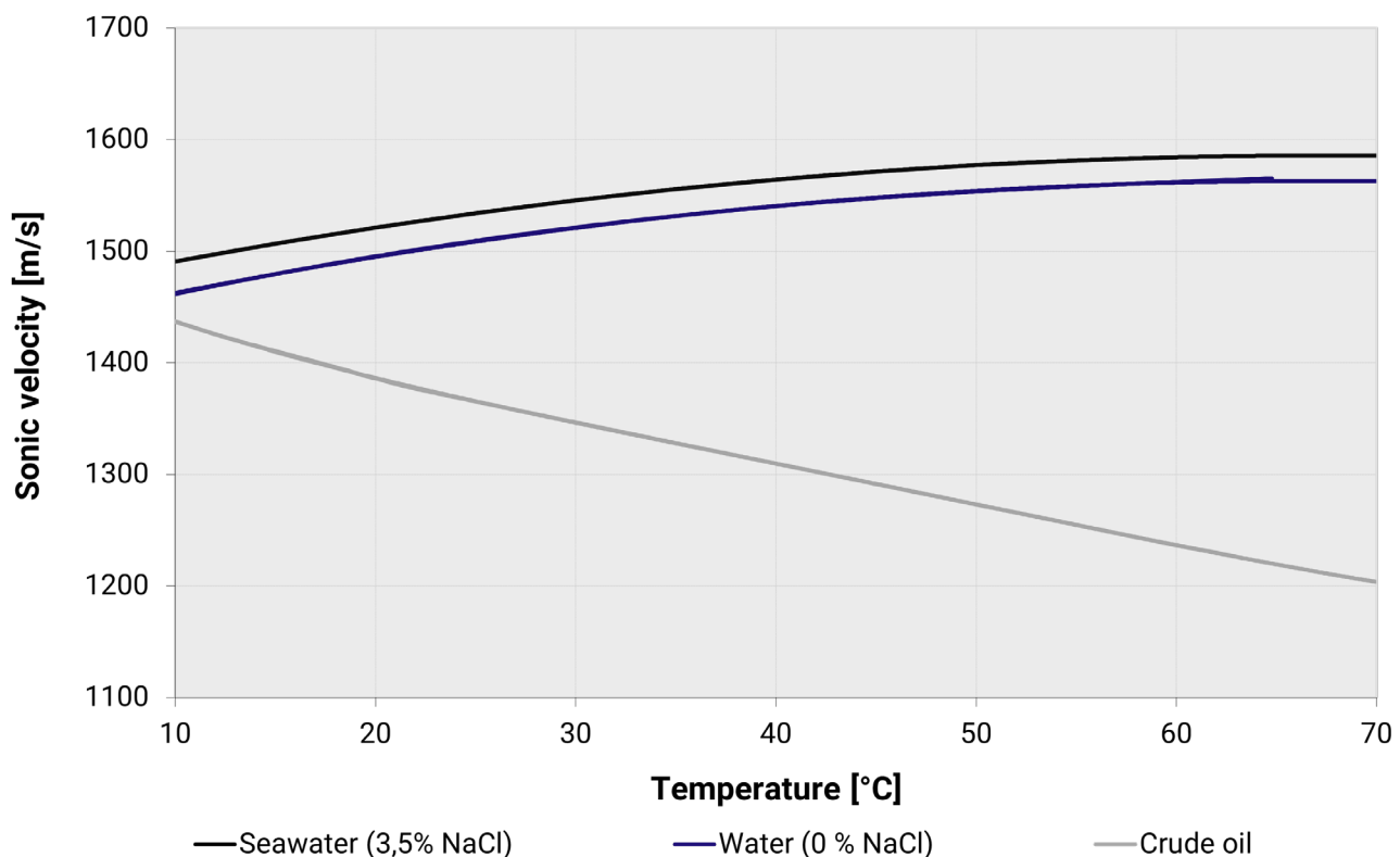
Phase separation by means of LiquiSonic® sonic velocity measurement
