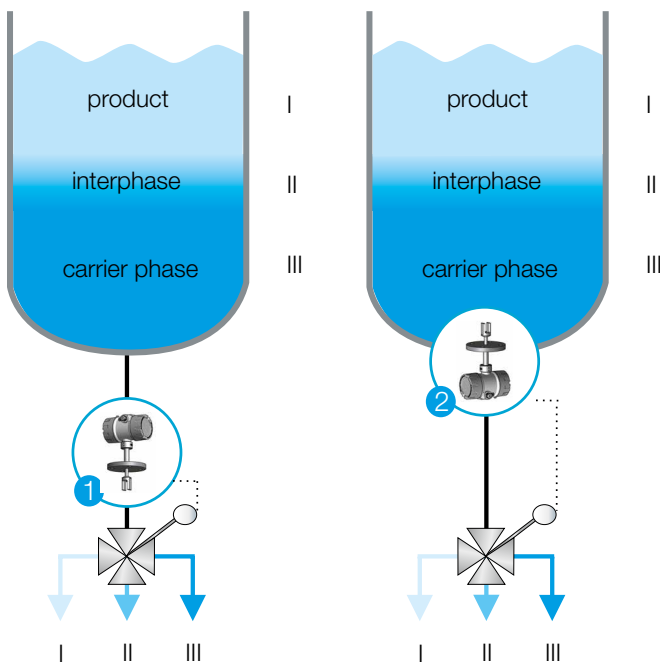
Phase separation in batch process
