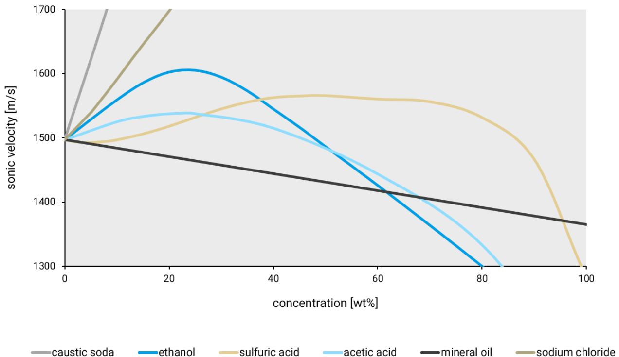
Correlation between sonic velocity and concentration of binary liquids
