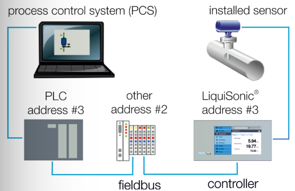
Connection interfaces
